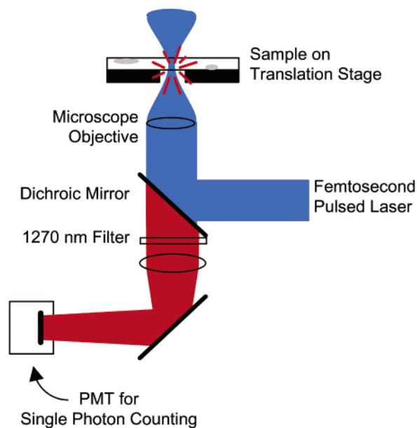
FIGURE 9. Illustration of the inverted microscope used to create singlet oxygen in and monitor singlet oxygen from a small focal volume upon two-photon irradiation of a sensitizer.
